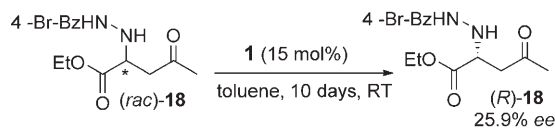
Scheme 2. Deracemization of racemic Mannich-product 18 .
